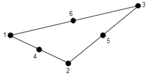
2-D quadratic element showing node numbering
