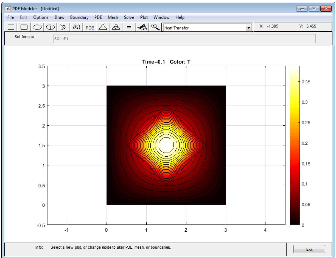
Isothermal Lines
